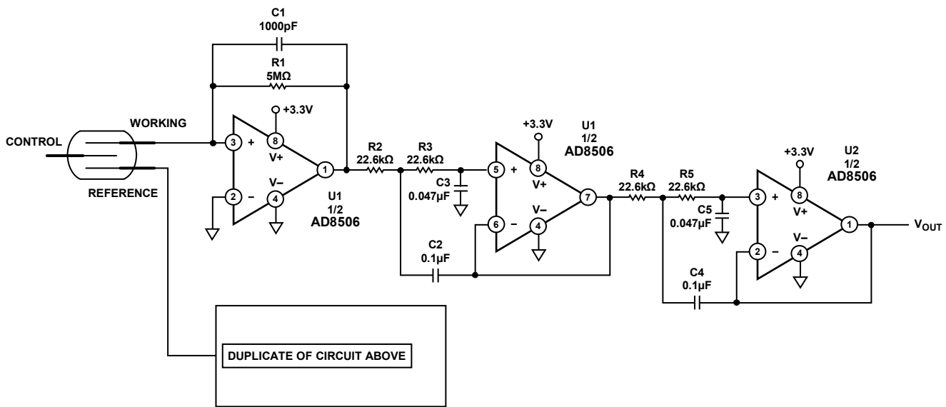
Figure 47. A Four-Pole Butterworth Filter That Can Be Used in a Glucose Meter
