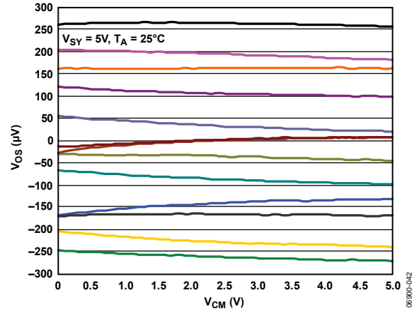
Figure 45. Input Offset Voltage vs. Input Common-Mode Voltage Response (Powered by a 5 V Supply; Results of 12 Units Are Displayed)
