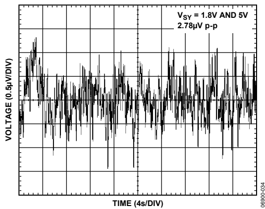
Figure 36. Voltage Noise 0.1 Hz to 10 Hz
