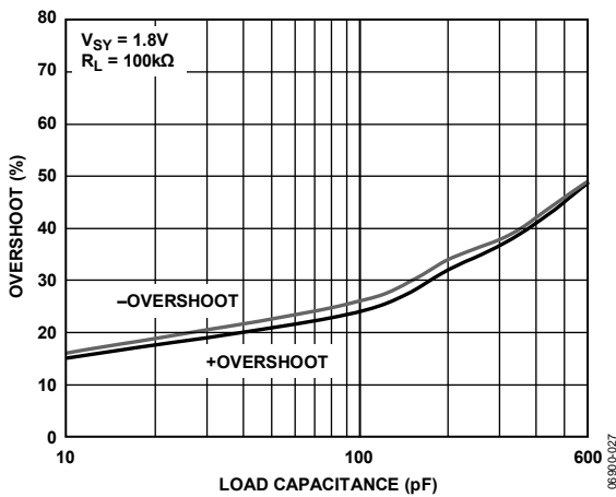
Figure 30. Small Signal Overshoot vs. Load Capacitance
