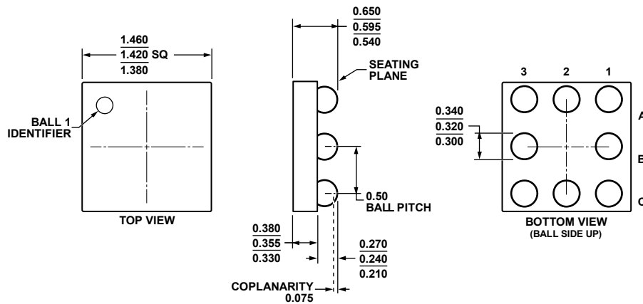
Figure 49. 8-Ball Wafer Level Chip Scale Package [WLCSP] (CB-8-2)
