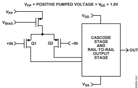
Figure 44. Typical Front-End Section of an Op Amp with Embedded Charge Pump
