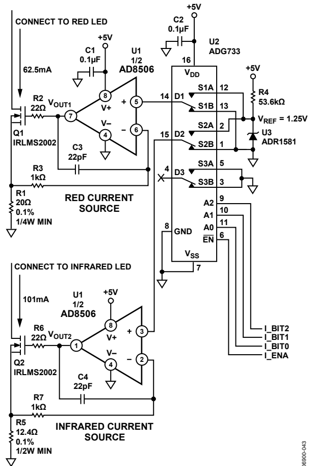
Figure 46. Pulse Oximeter Red and Infrared Current Sources Using the AD8506 as a Buffer to the Voltage Reference Device
