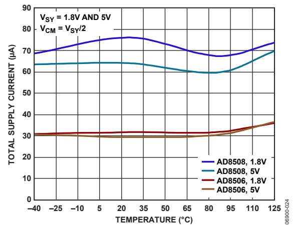
Figure 21. Total Supply Current vs. Temperature
