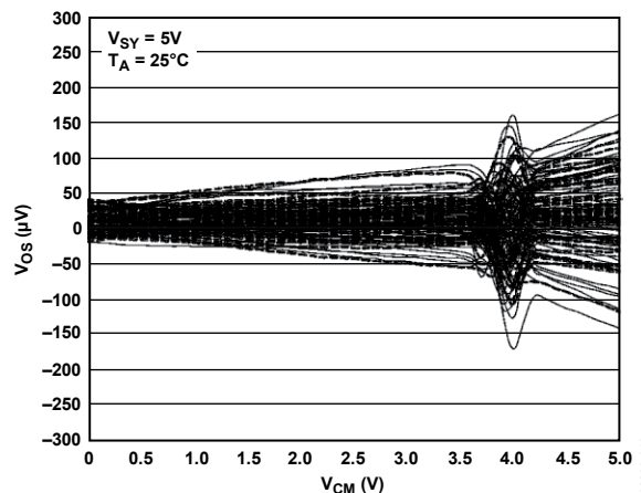
Figure 43. Typical Input Offset Voltage vs. Common-Mode Voltage Response in a Dual Differential Pair Input Stage Op Amp (Powered by 5 V Supply; Results of Approximately 100 Units per Graph Are Displayed)
