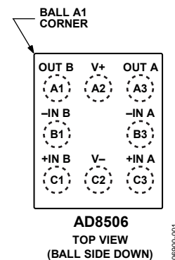
Figure 2. 8-Ball WLCSP (CB-8-2)
