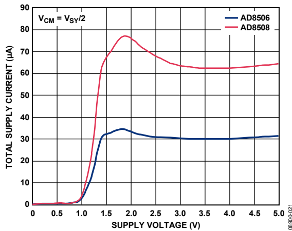
Figure 18. Total Supply Current vs. Supply Voltage
